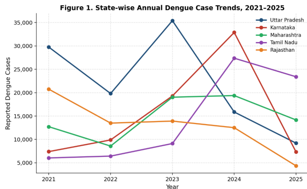
Figure 1. State-wise annual dengue case trends, 2021–2025 (source: NCVBDC surveillance data [4]).
