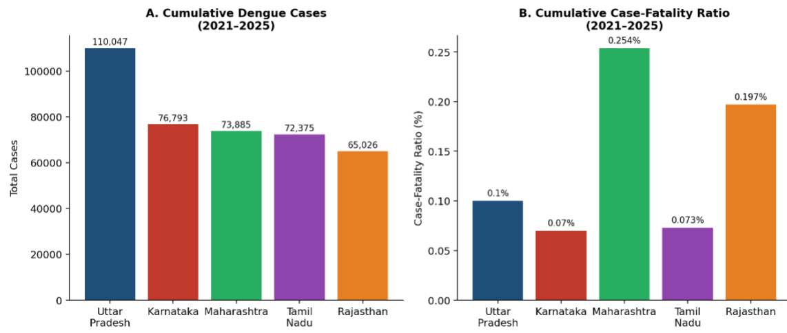
Figure 2. Cumulative dengue case burden (Panel A) and case-fatality ratio (Panel B) by state, 2021–2025 (source: NCVBDC surveillance data [4]).
