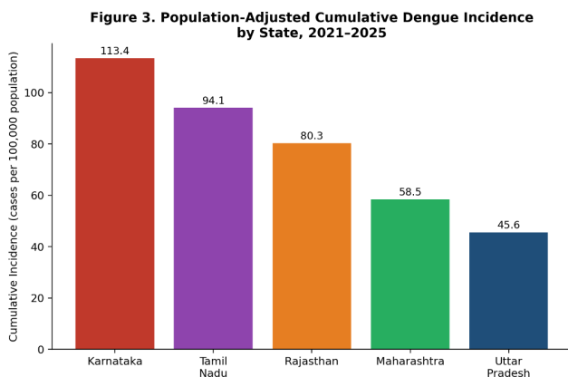
Figure 3. Population-adjusted cumulative dengue incidence by state, 2021–2025 (cases per 100,000 population, derived from NCVBDC surveillance data [4] and 2025 population projections [16]).
